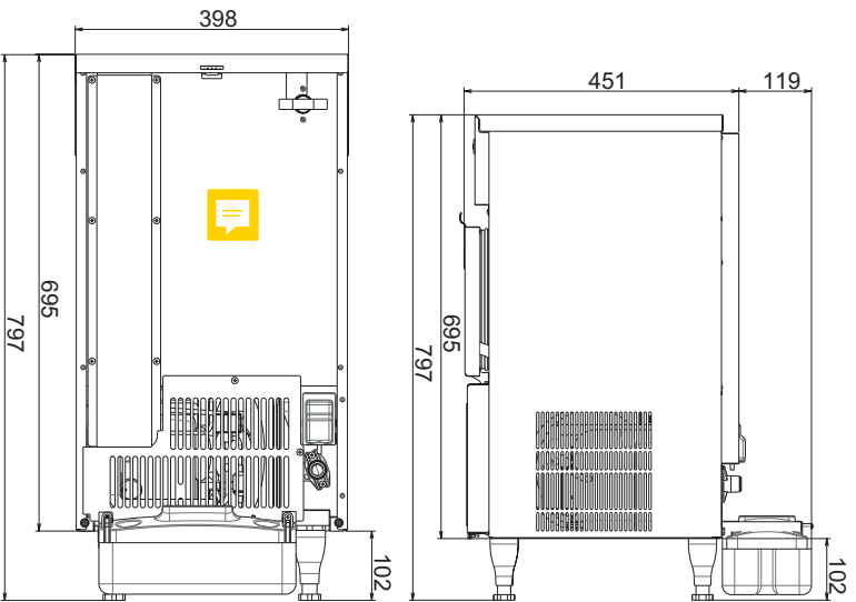
PUMP POSITION AT REAR
