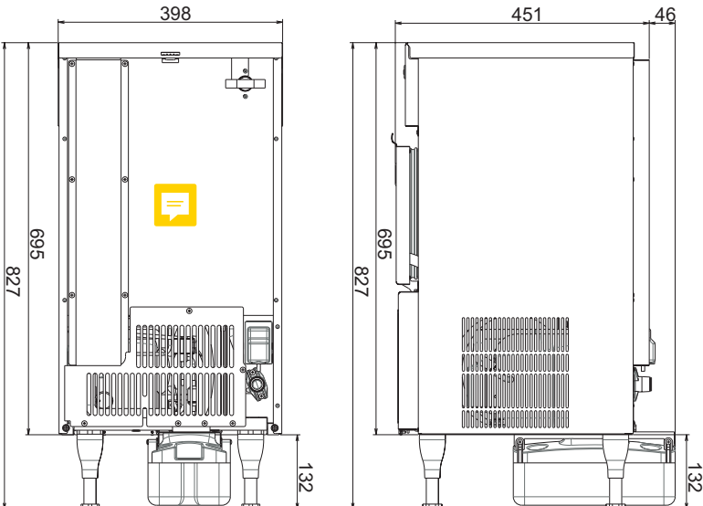
PUMP POSITION UNDERNEATH
